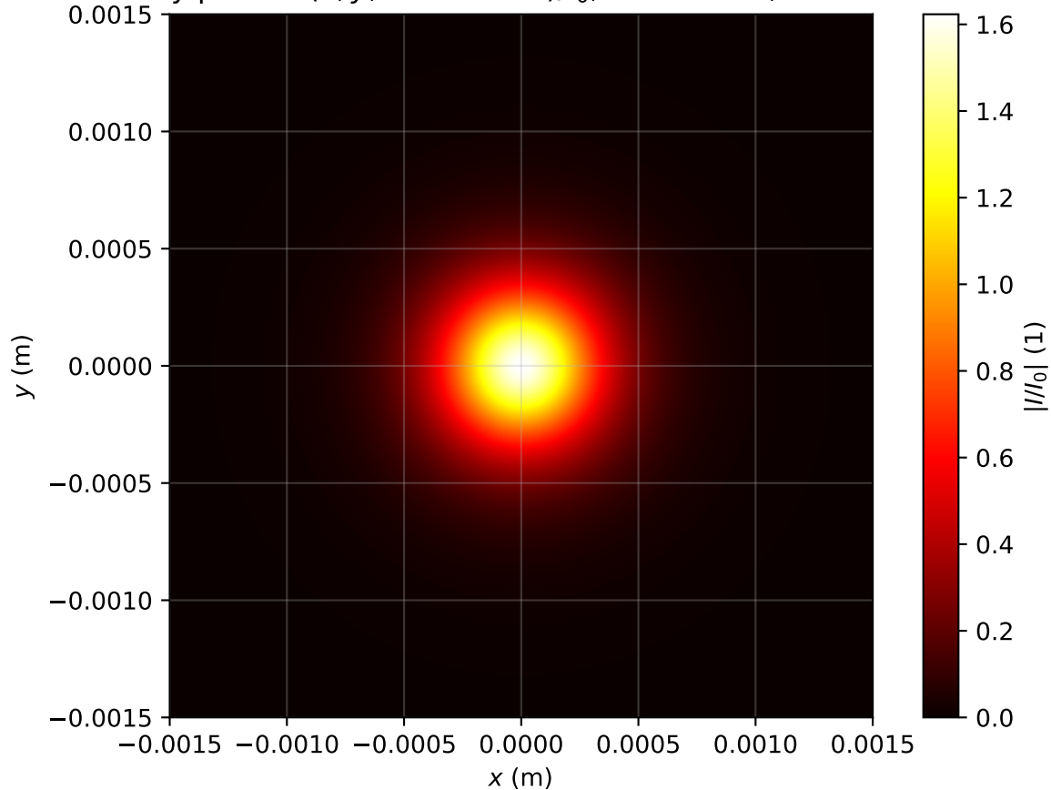
Intensity profile I(x, y, z = 2.468m)/I_0 , \text{Pin}=0.9\text{Pcr} , artificial time
